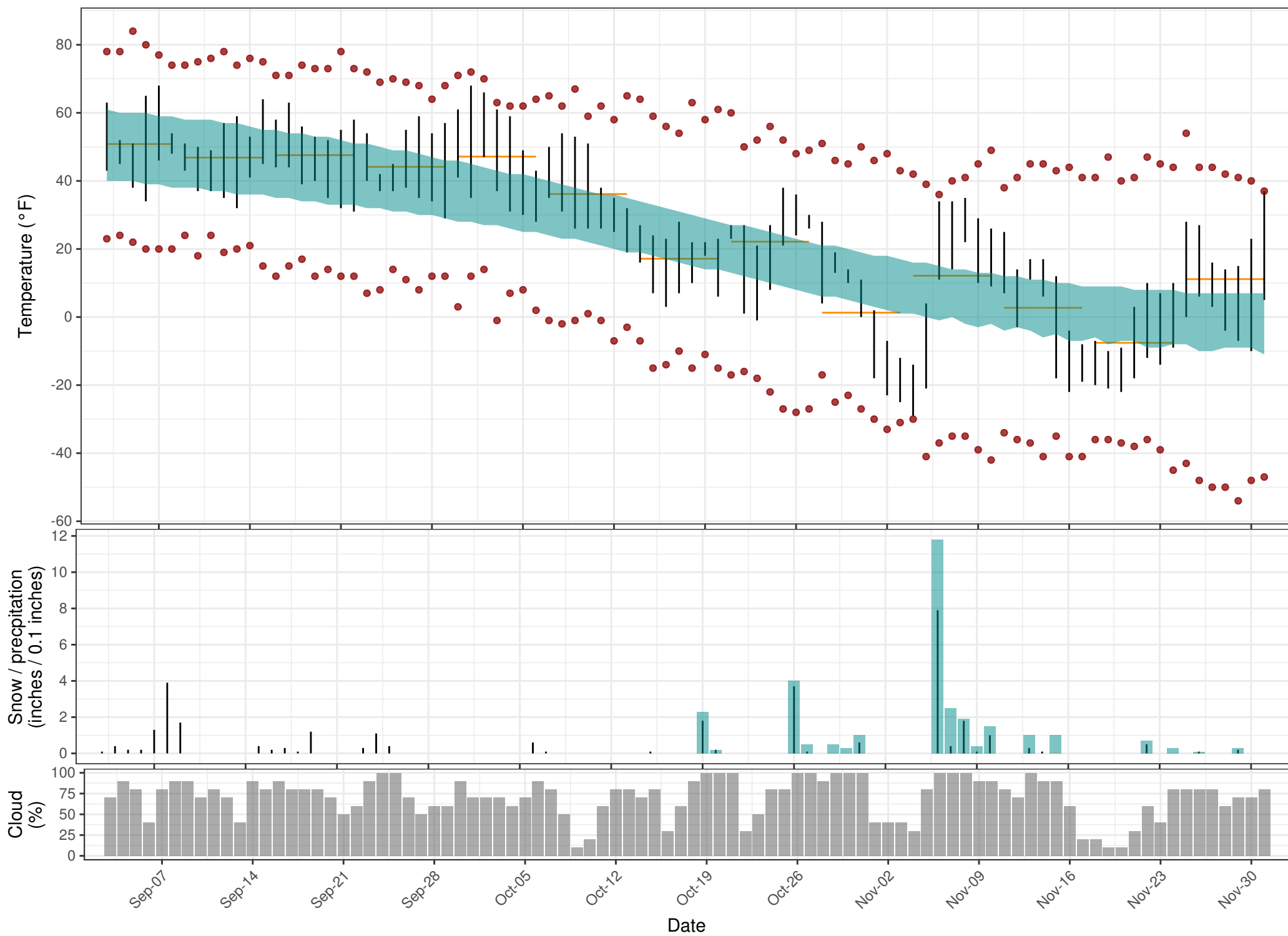
Daily temperature, precipitation and cloud cover, Fairbanks Airport (PAFA) 2020
