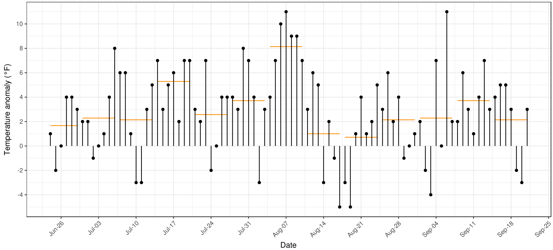
Difference between daily mean temperature and 30-year average, Fairbanks Airport (PAFA) 2017
