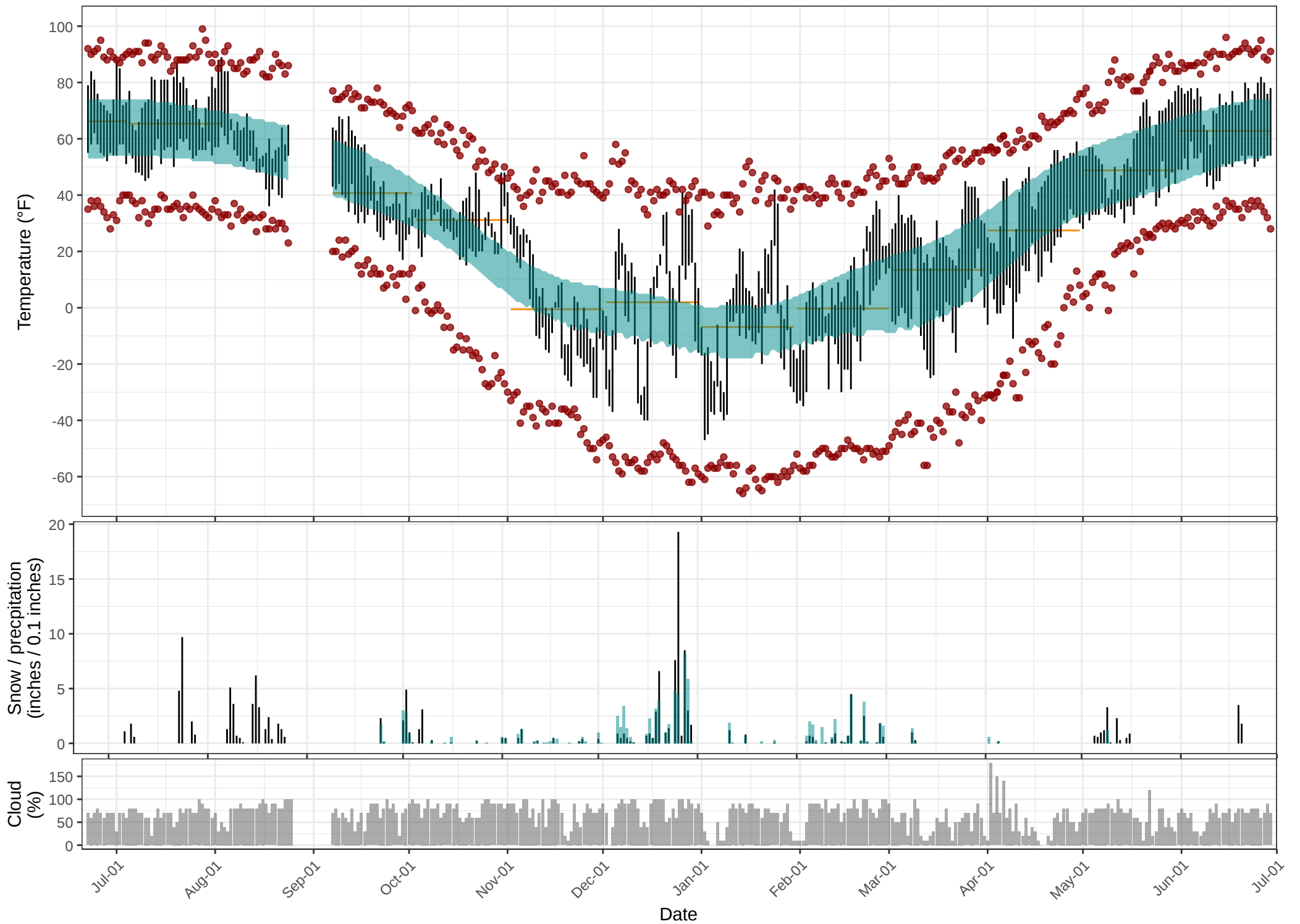
Daily temperature, precipitation and cloud cover, Fairbanks Airport (PAFA) 2021–2022
